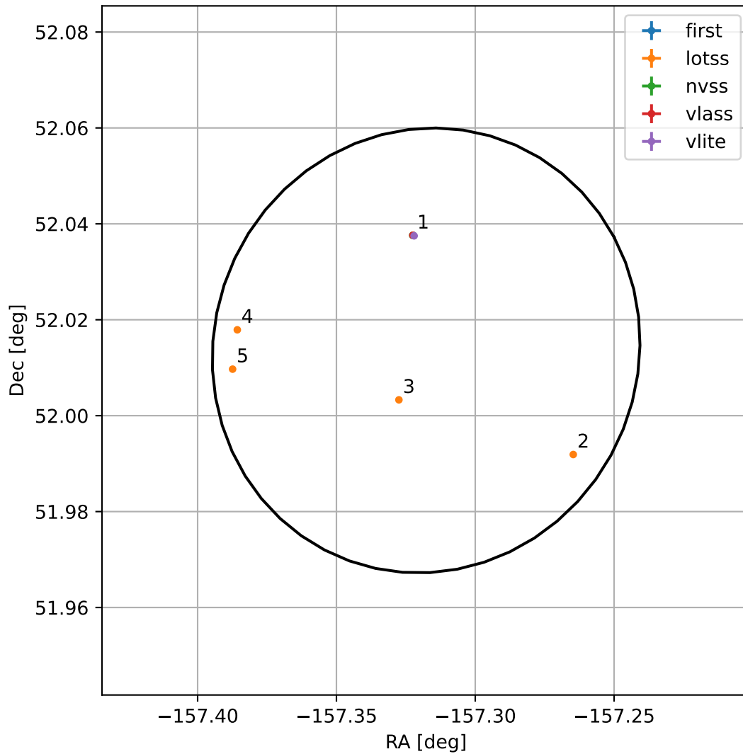
4FGL J1330.7+5200
