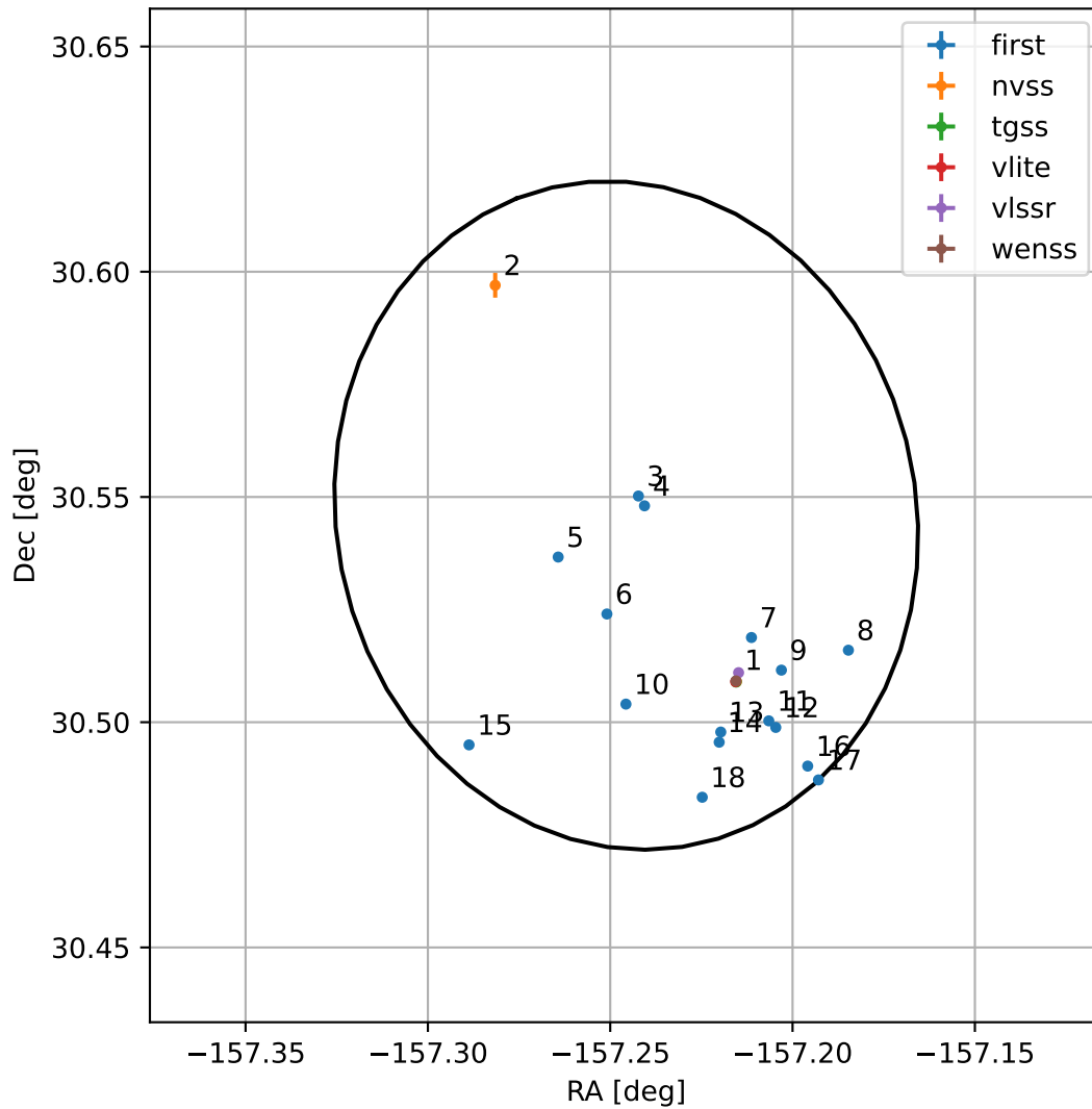
4FGL J1331.0+3032
