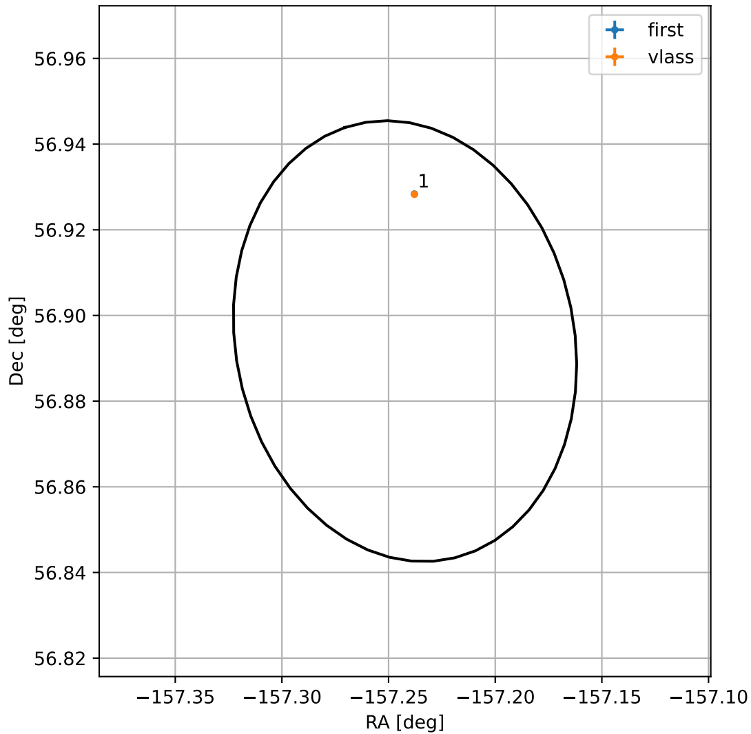
4FGL J1331.0+5653
