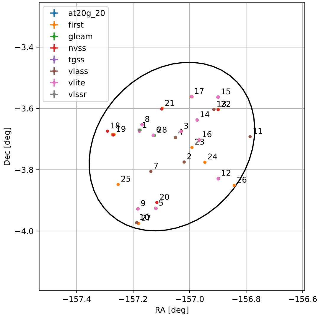
4FGL J1331.7-0343
