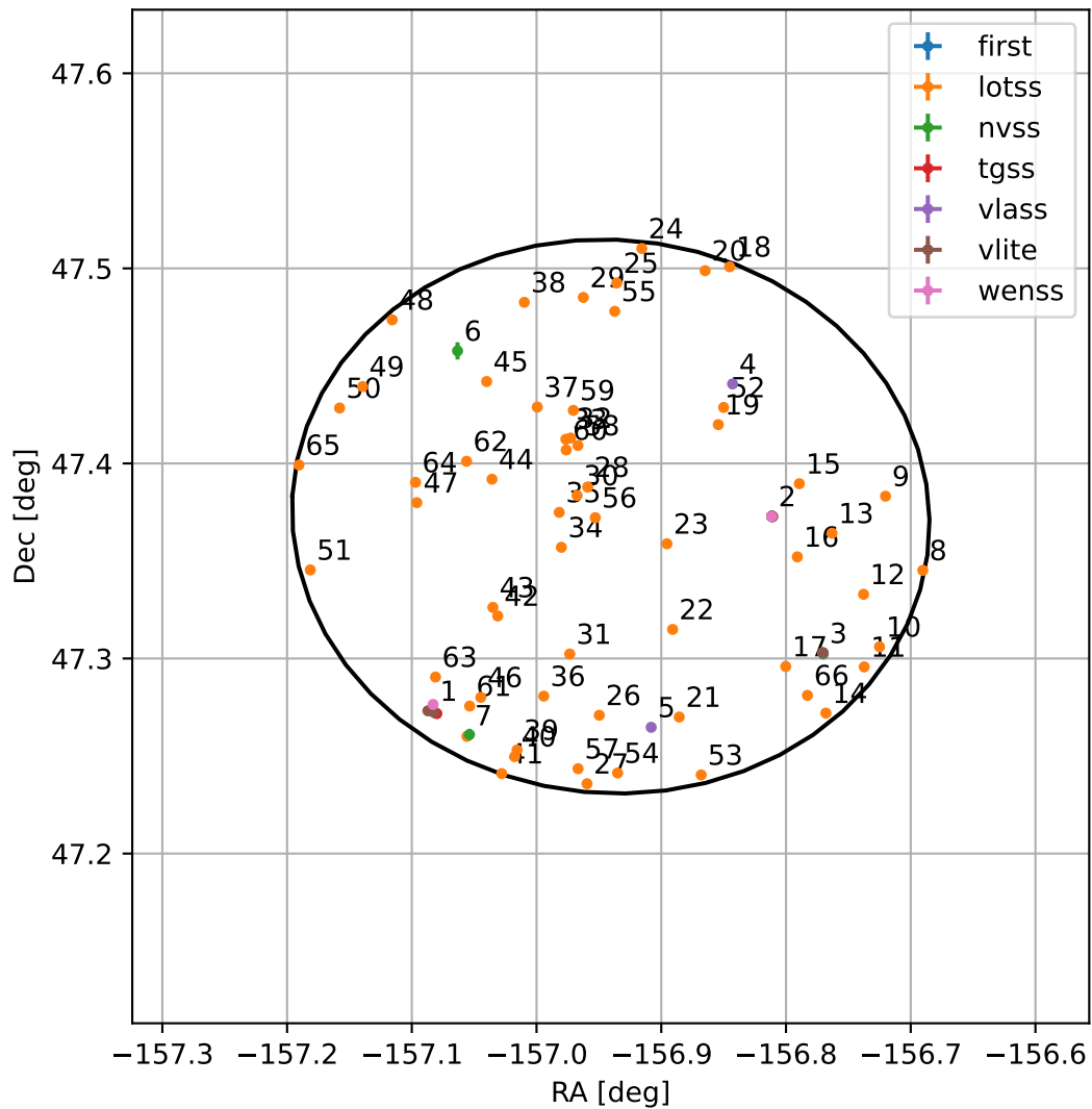
4FGL J1332.2+4722
