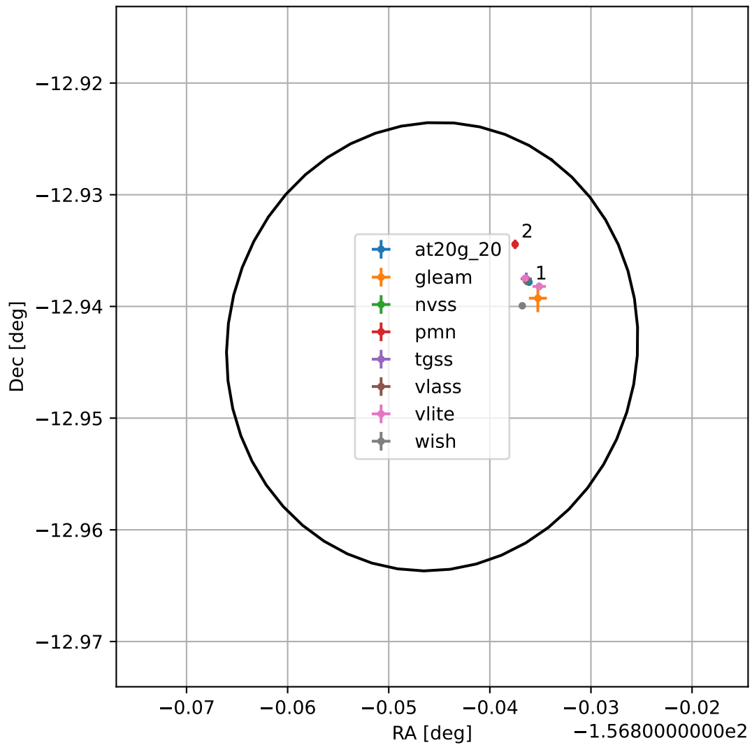
4FGL J1332.6-1256
