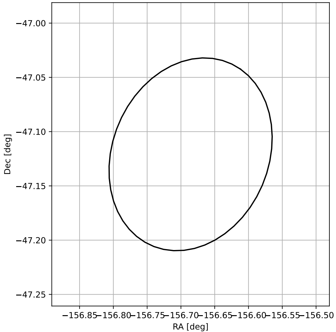
4FGL J1333.2-4707
