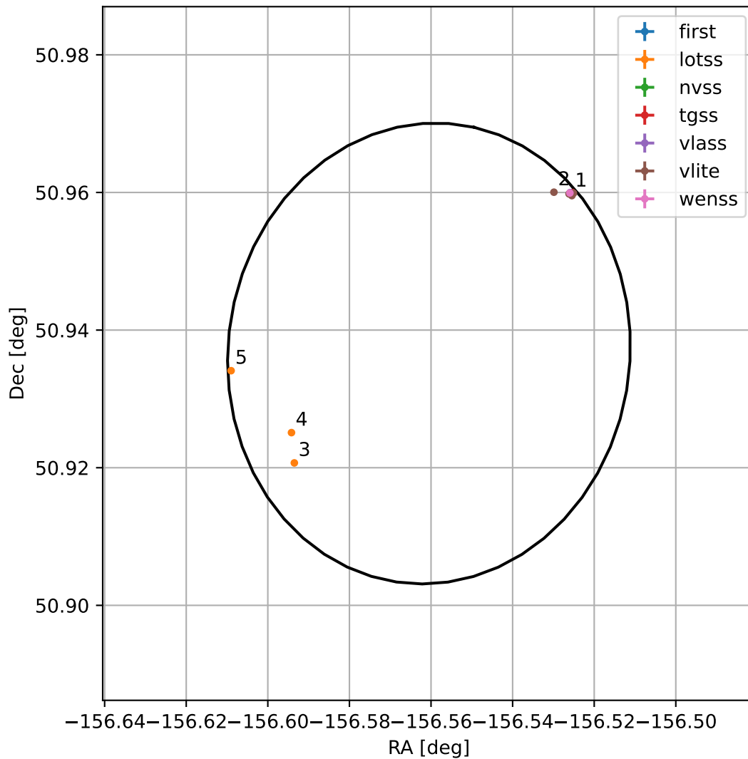
4FGL J1333.7+5056
