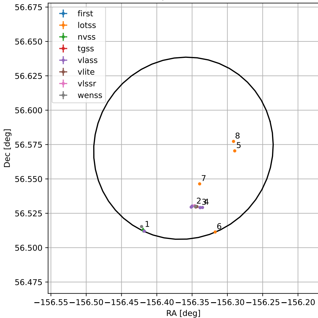
4FGL J1334.5+5634
