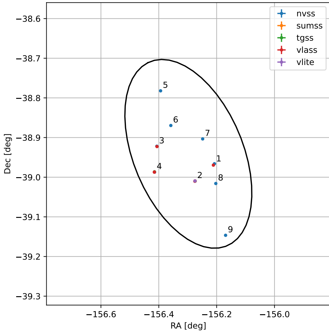
4FGL J1334.8-3856
