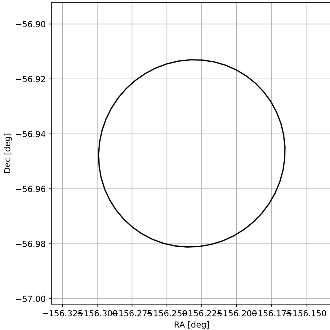
4FGL J1335.0-5656
