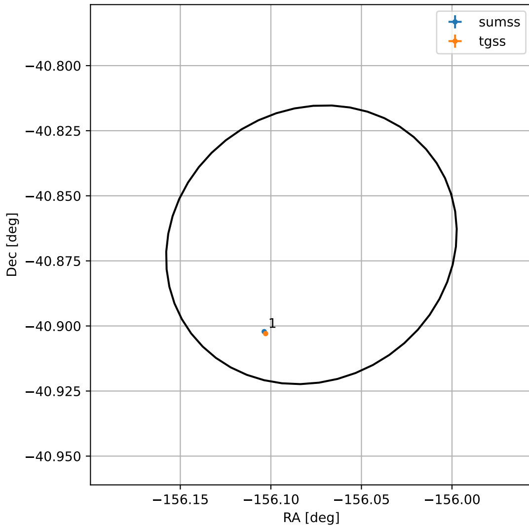
4FGL J1335.6-4052
