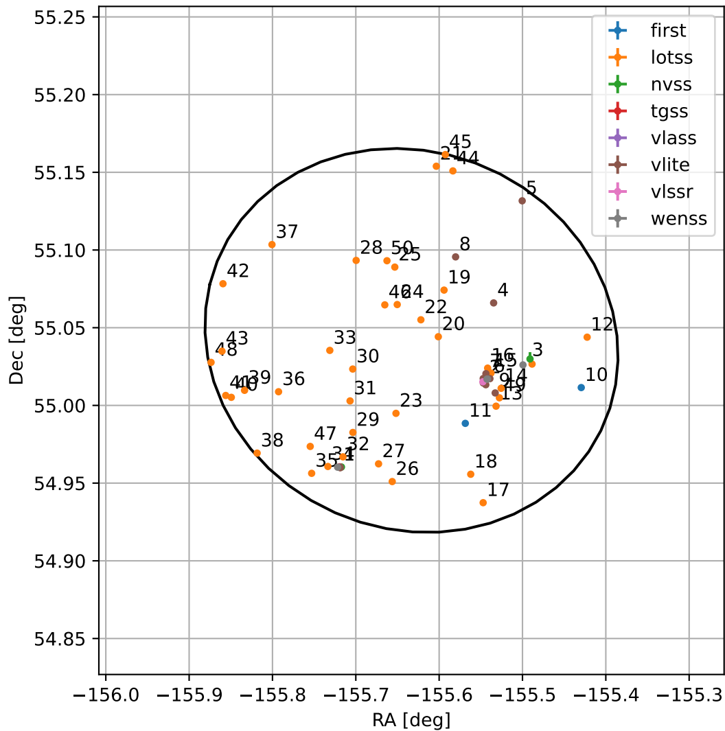
4FGL J1337.4+5502
