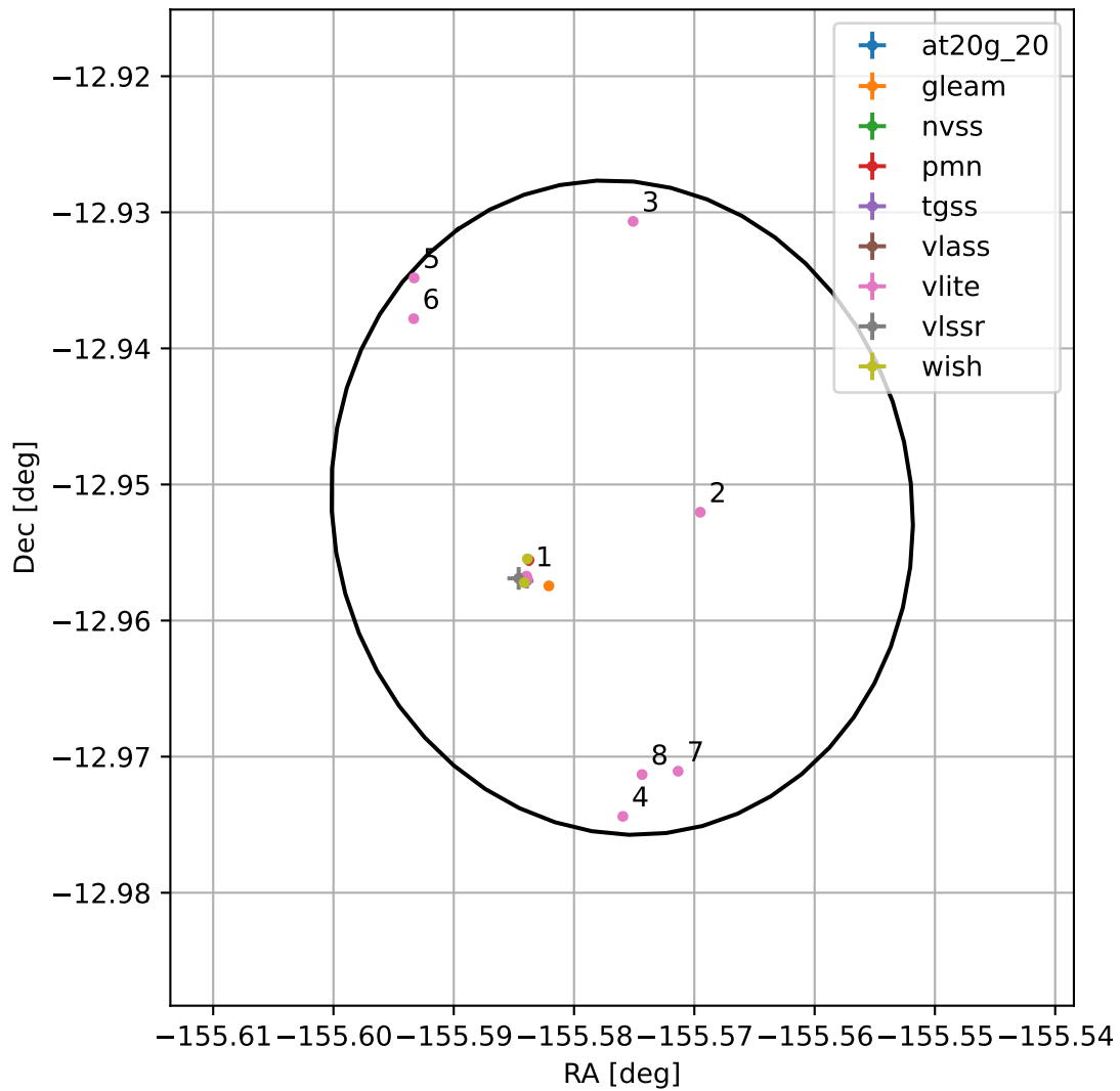
4FGL J1337.6-1257
