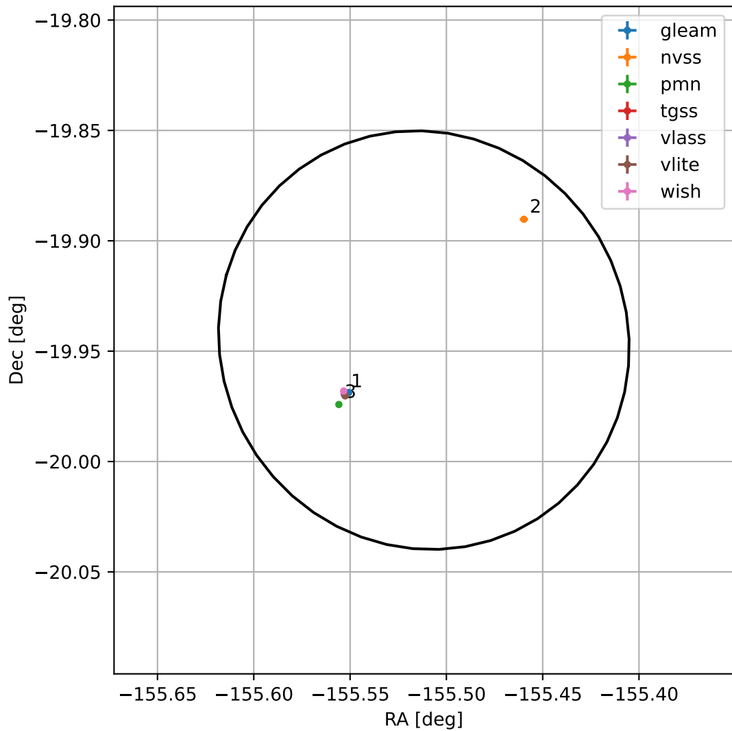
4FGL J1337.9-1956
