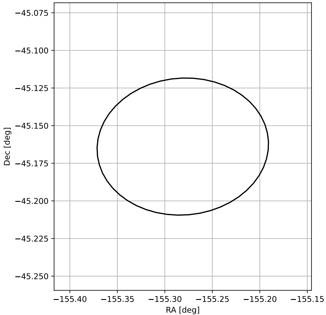
4FGL J1338.8-4509
