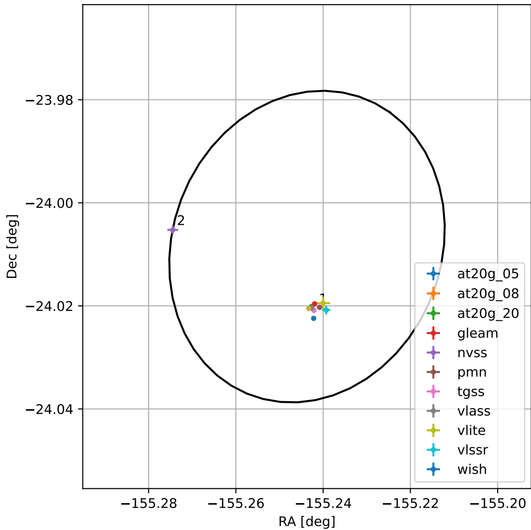
4FGL J1339.0-2400
