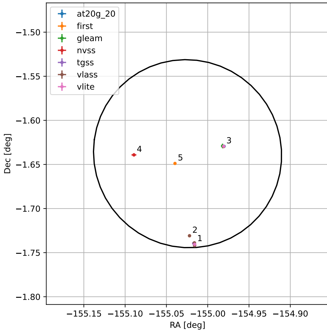
4FGL J1339.9-0138
