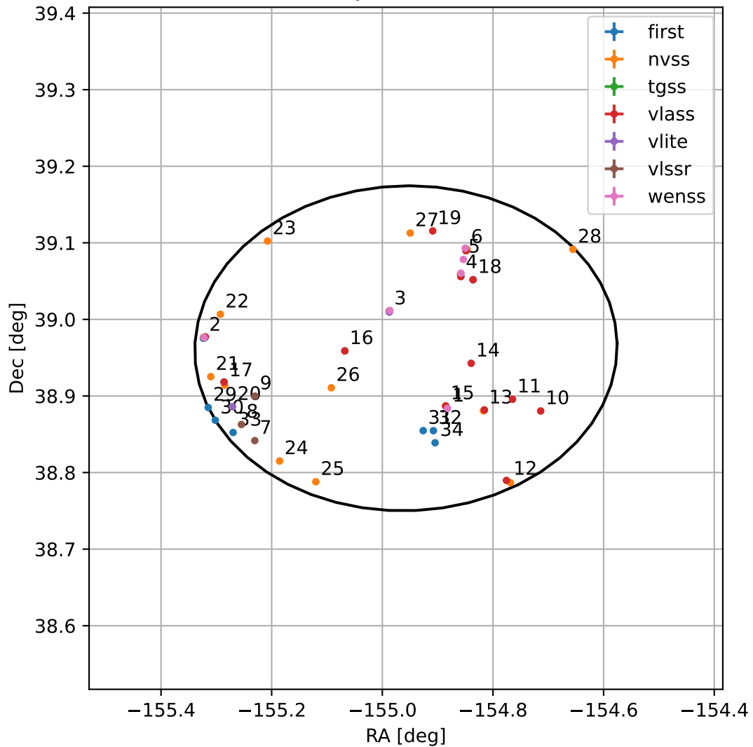
4FGL J1340.1+3857
