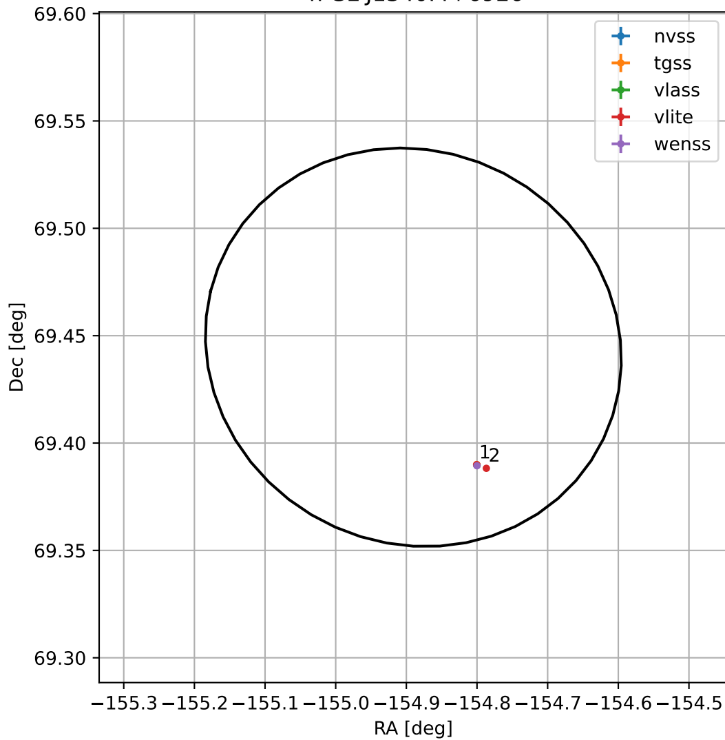
4FGL J1340.4+6926
