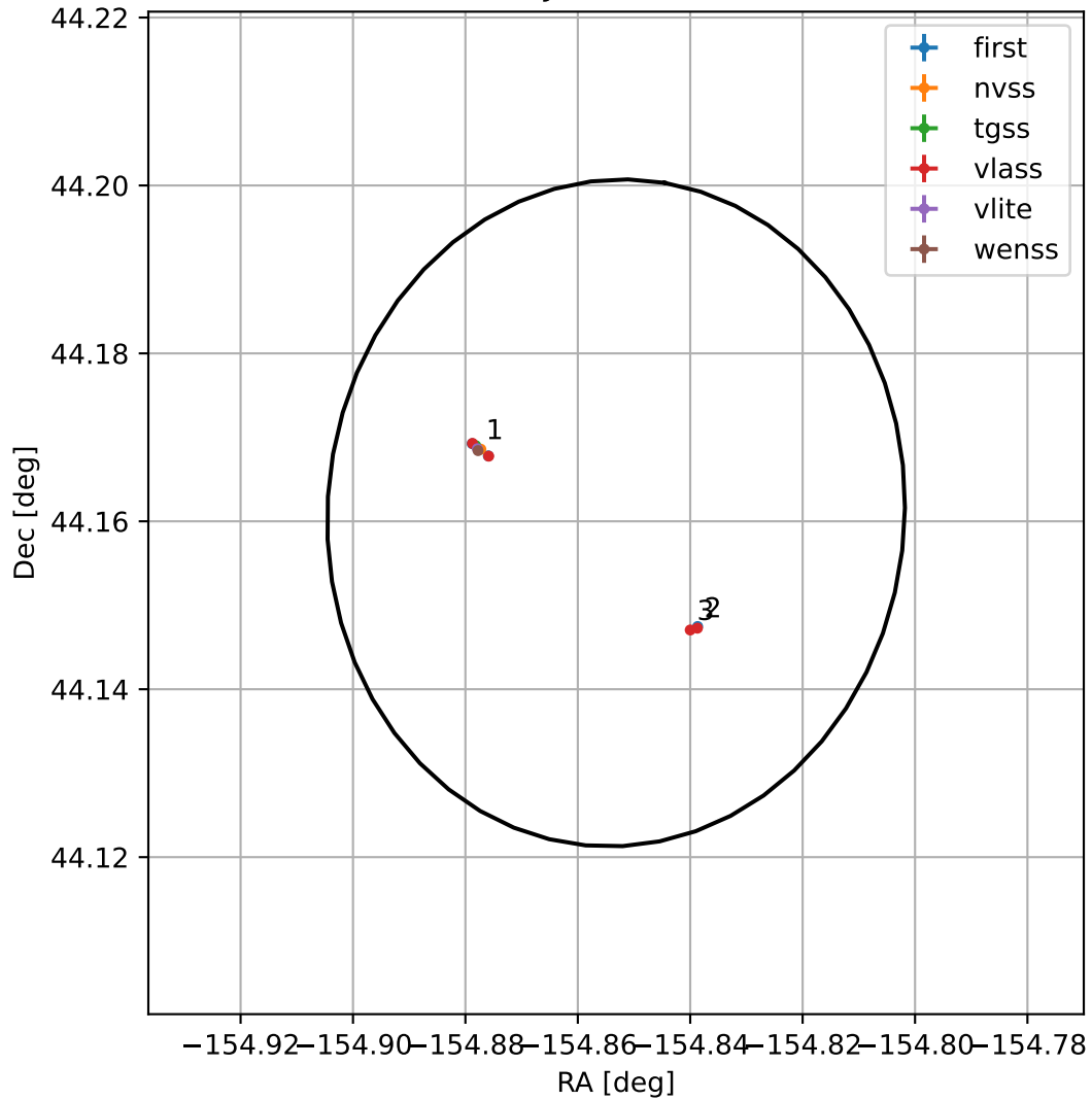
4FGL J1340.5+4409
