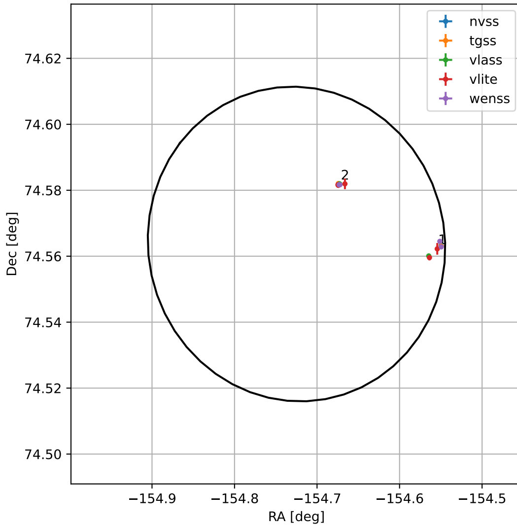
4FGL J1341.1+7433
