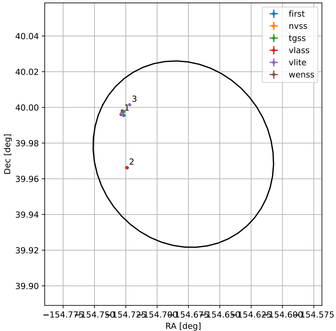
4FGL J1341.2+3958
