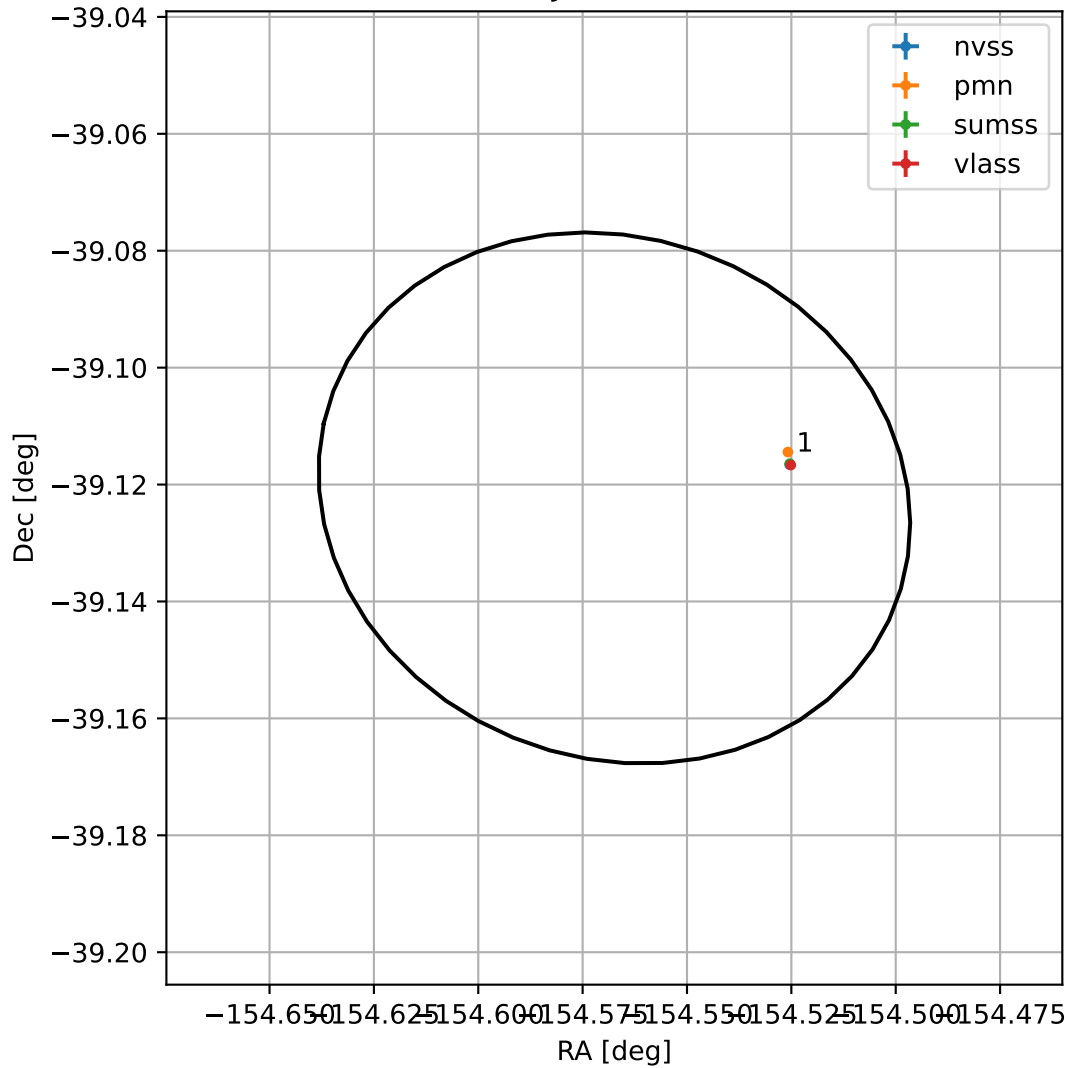
4FGL J1341.7-3907
