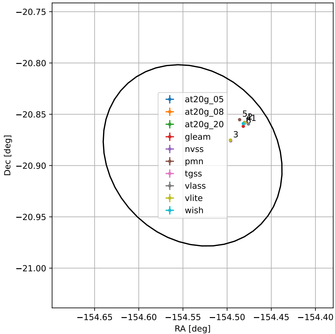
4FGL J1341.8-2053
