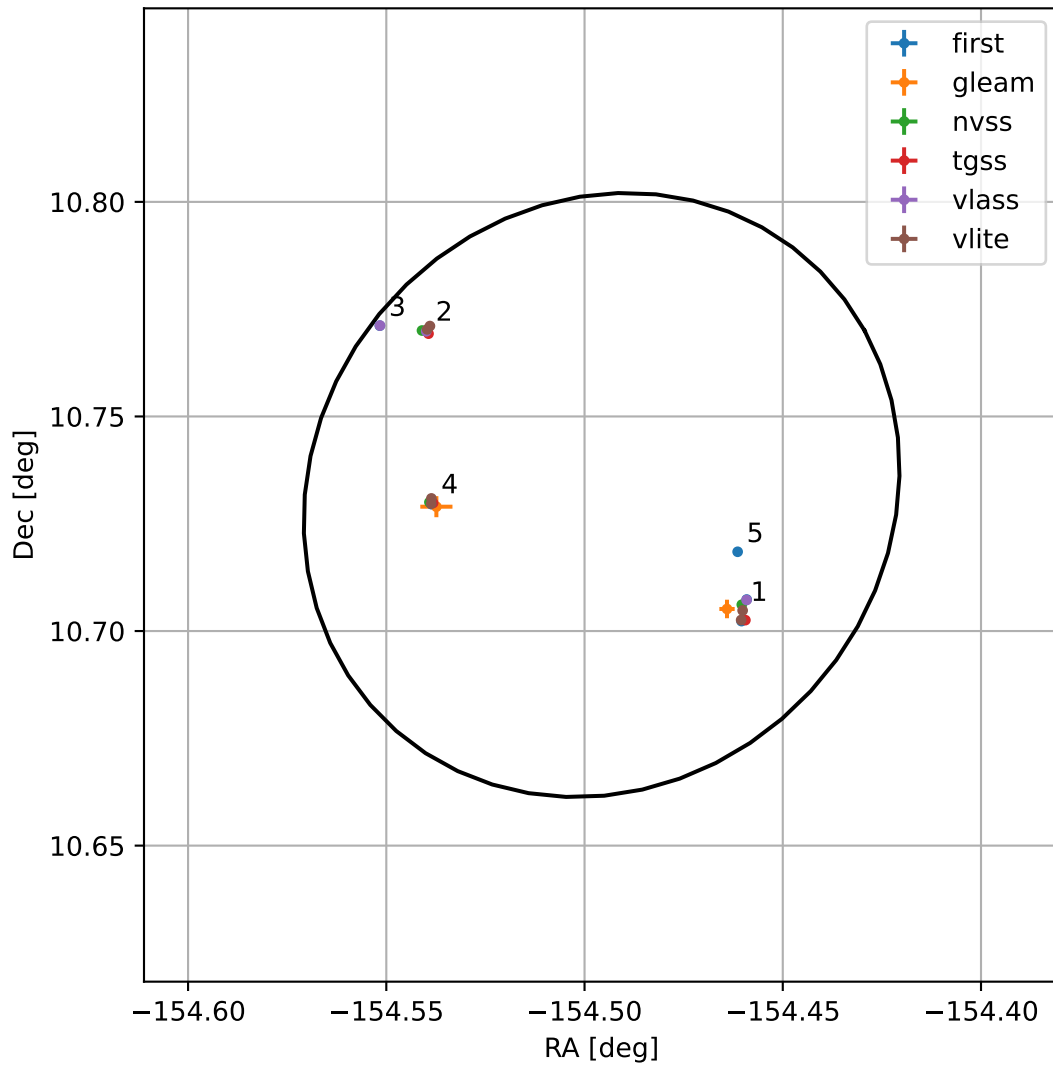
4FGL J1342.0+1043
