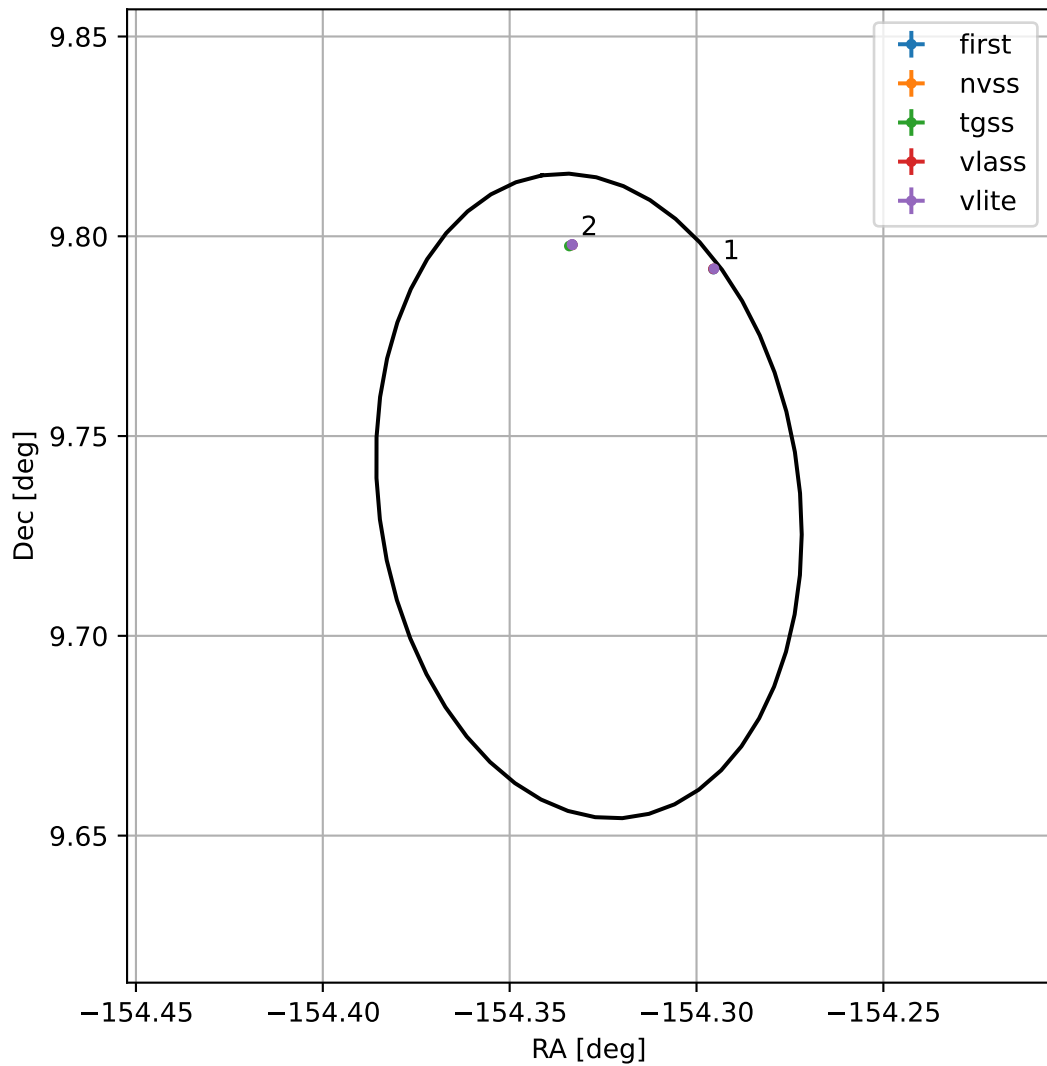
4FGL J1342.6+0944
