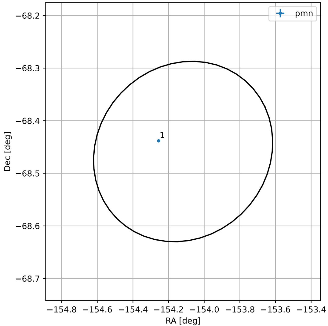
4FGL J1343.5-6827
