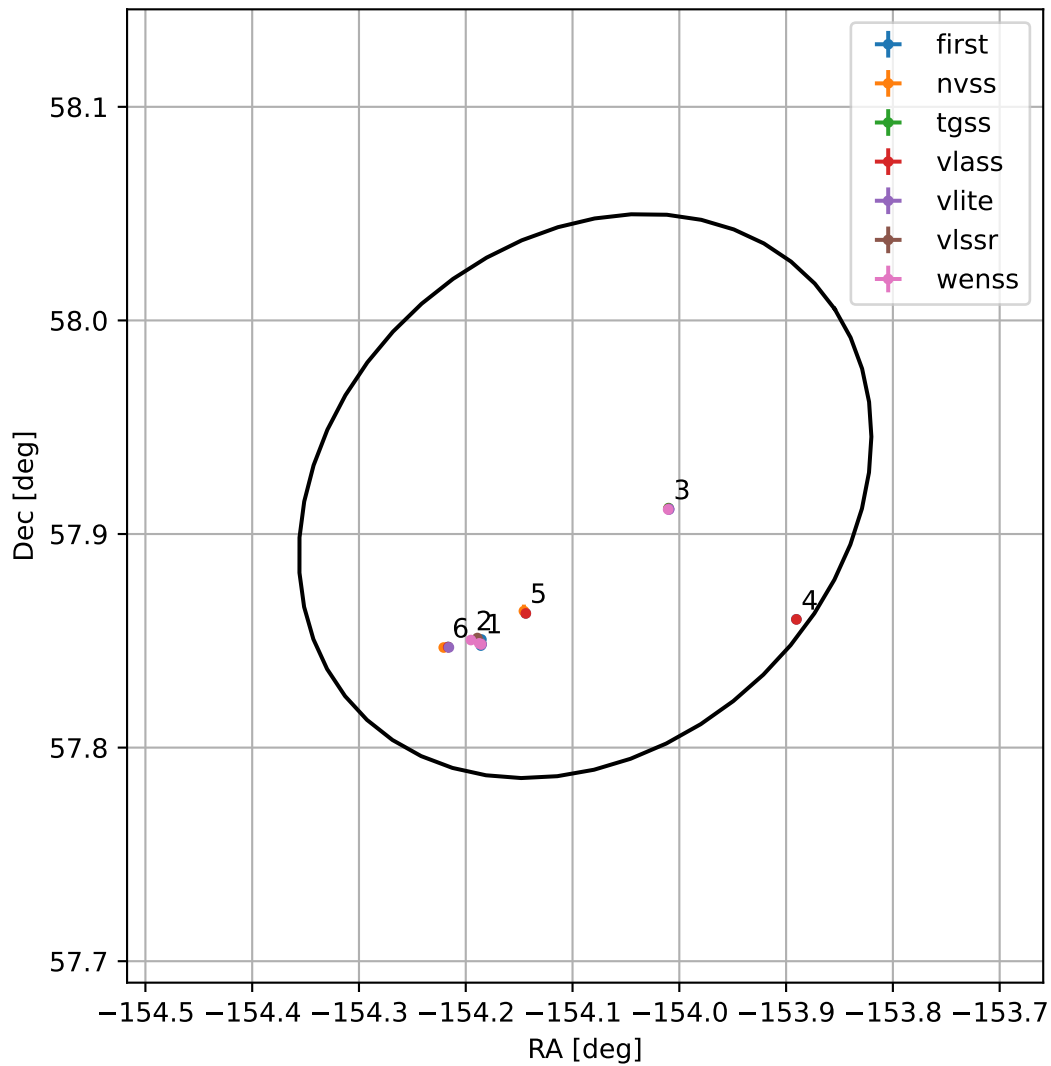
4FGL J1343.6+5755
