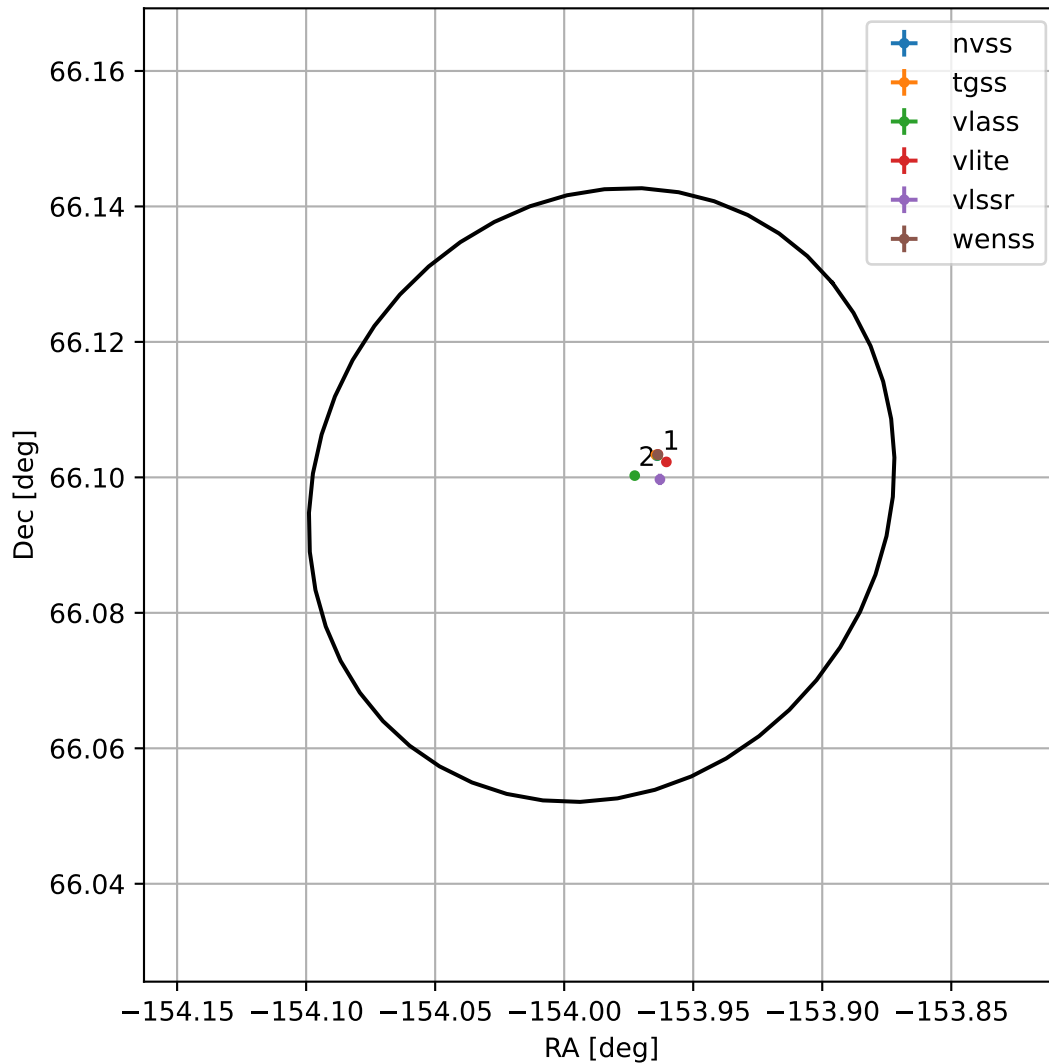
4FGL J1344.0+6605
