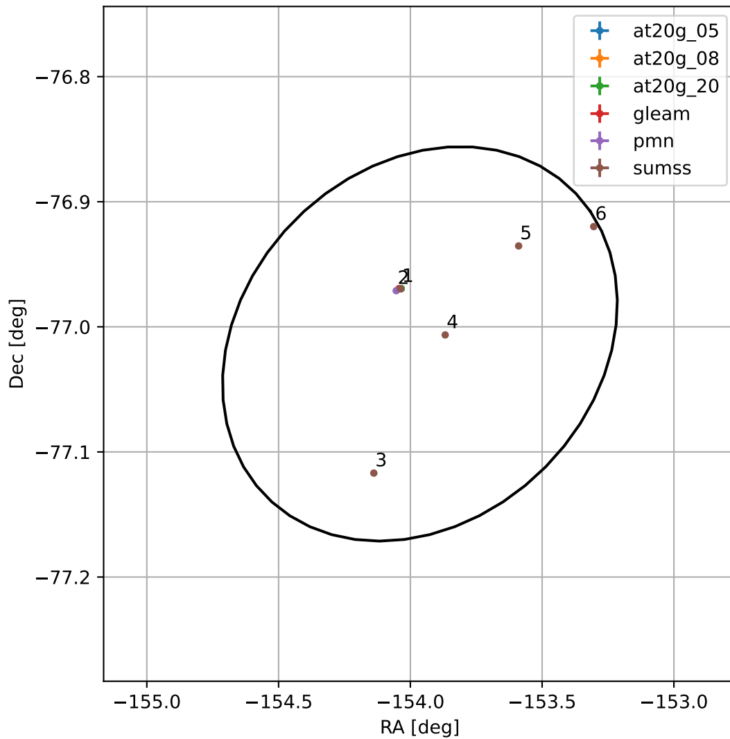
4FGL J1344.1-7700
