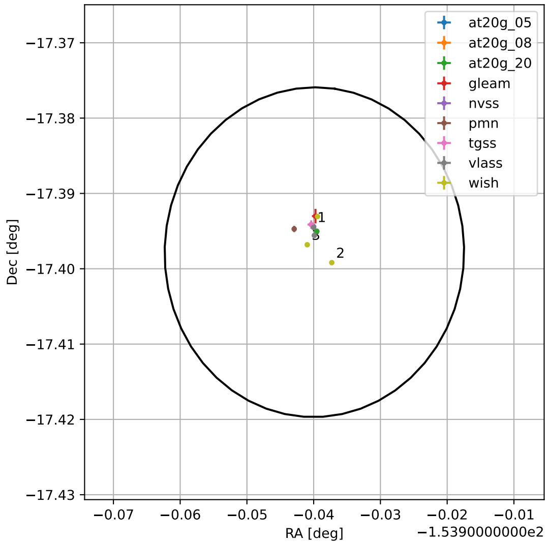
4FGL J1344.2-1723
