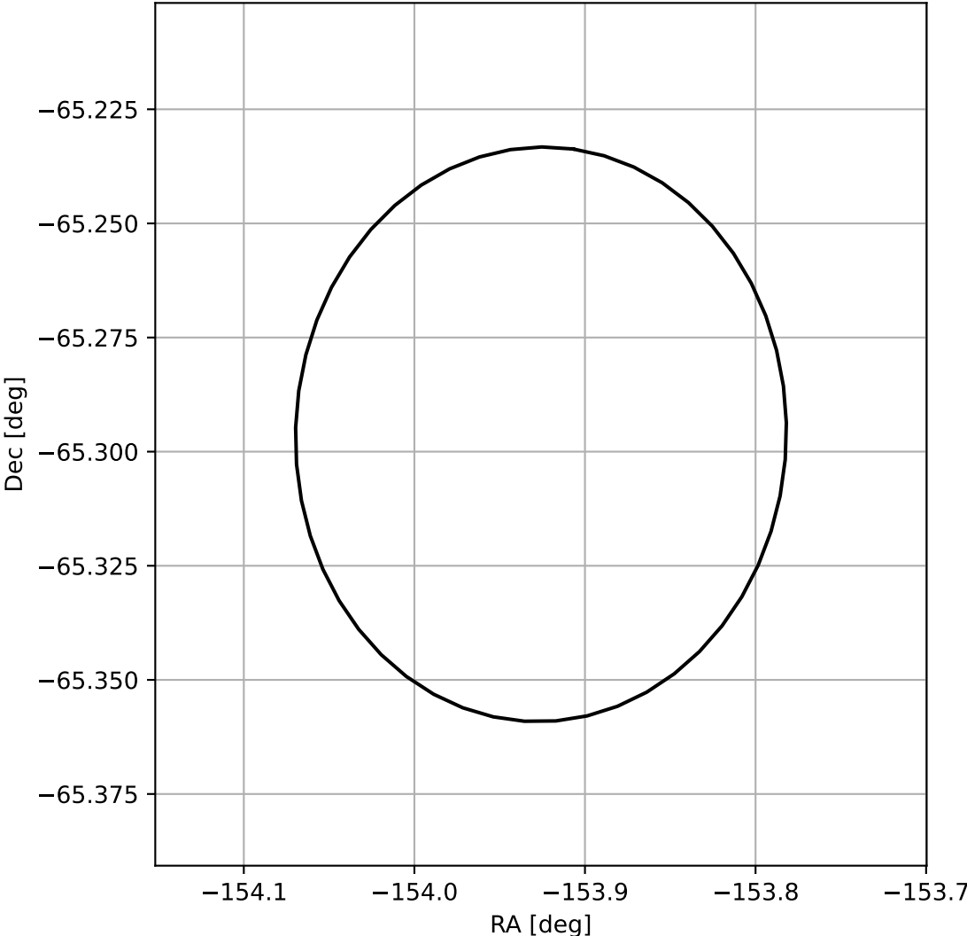
4FGL J1344.2-6517
