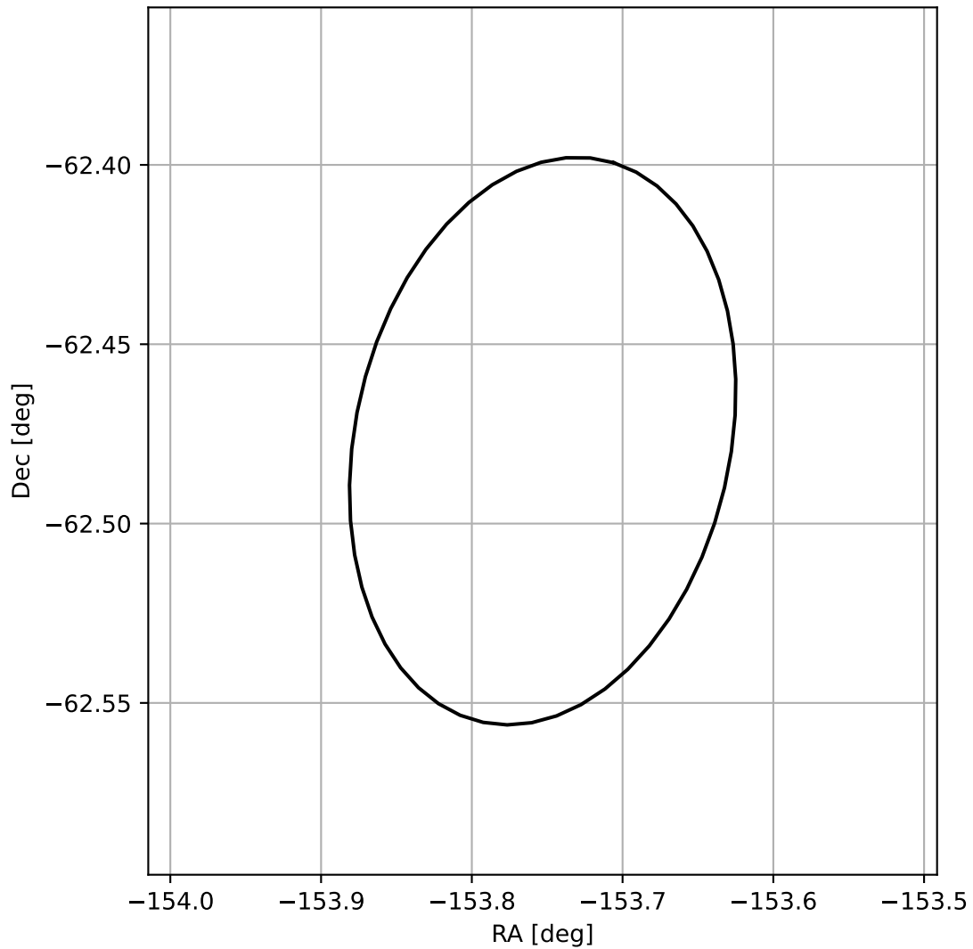
4FGL J1344.9-6228
