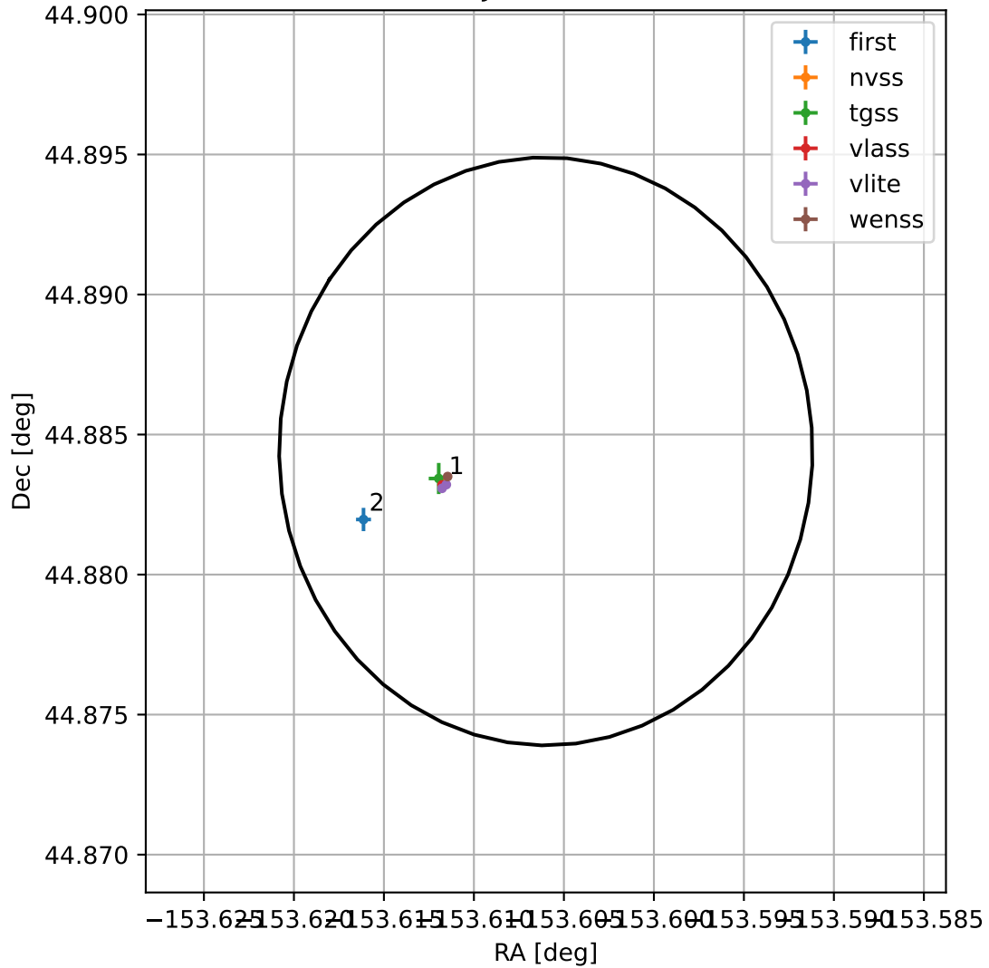
4FGL J1345.5+4453
