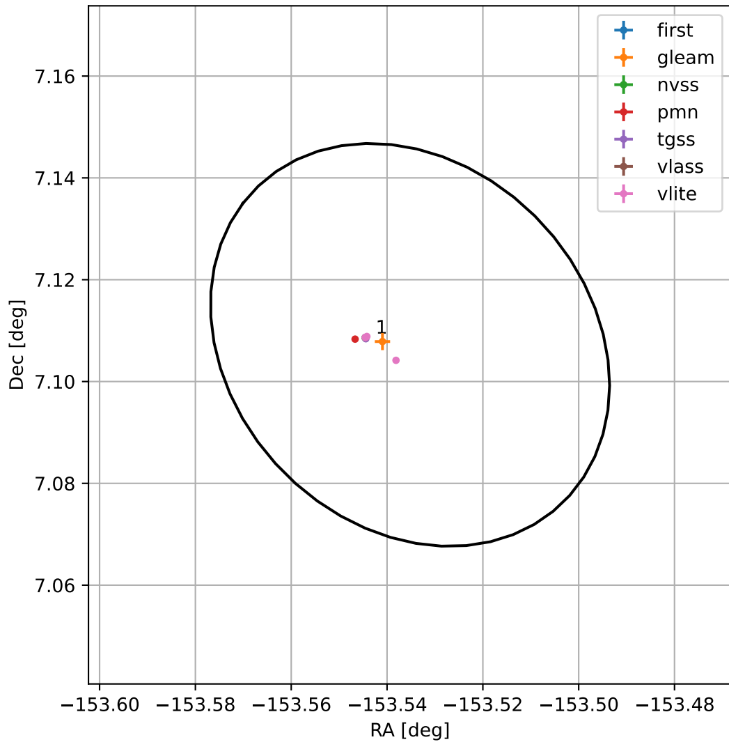
4FGL J1345.8+0706
