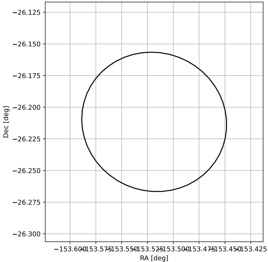
4FGL J1345.9-2612
