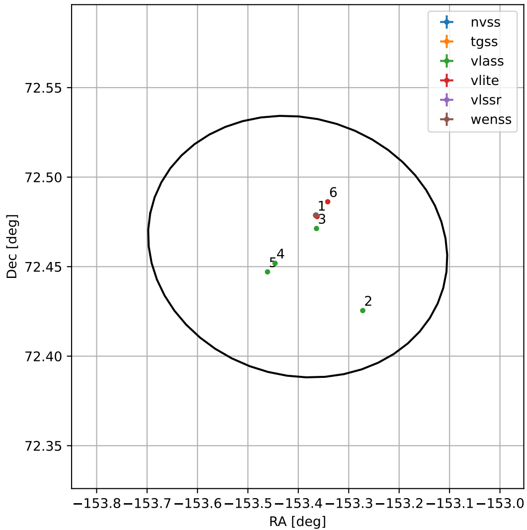
4FGL J1346.3+7227
