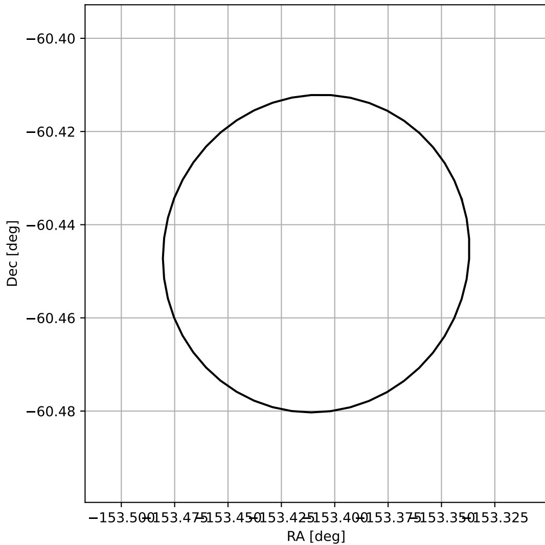
4FGL J1346.3-6026
