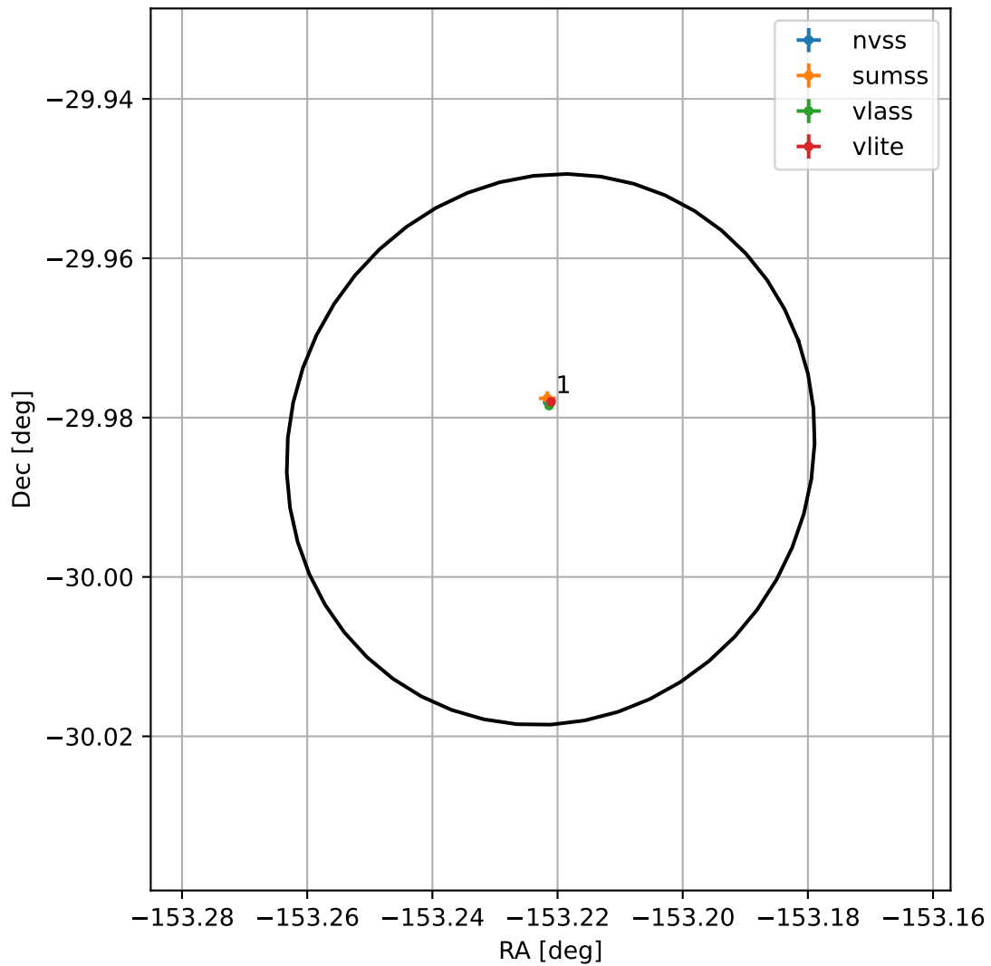
4FGL J1347.1-2959
