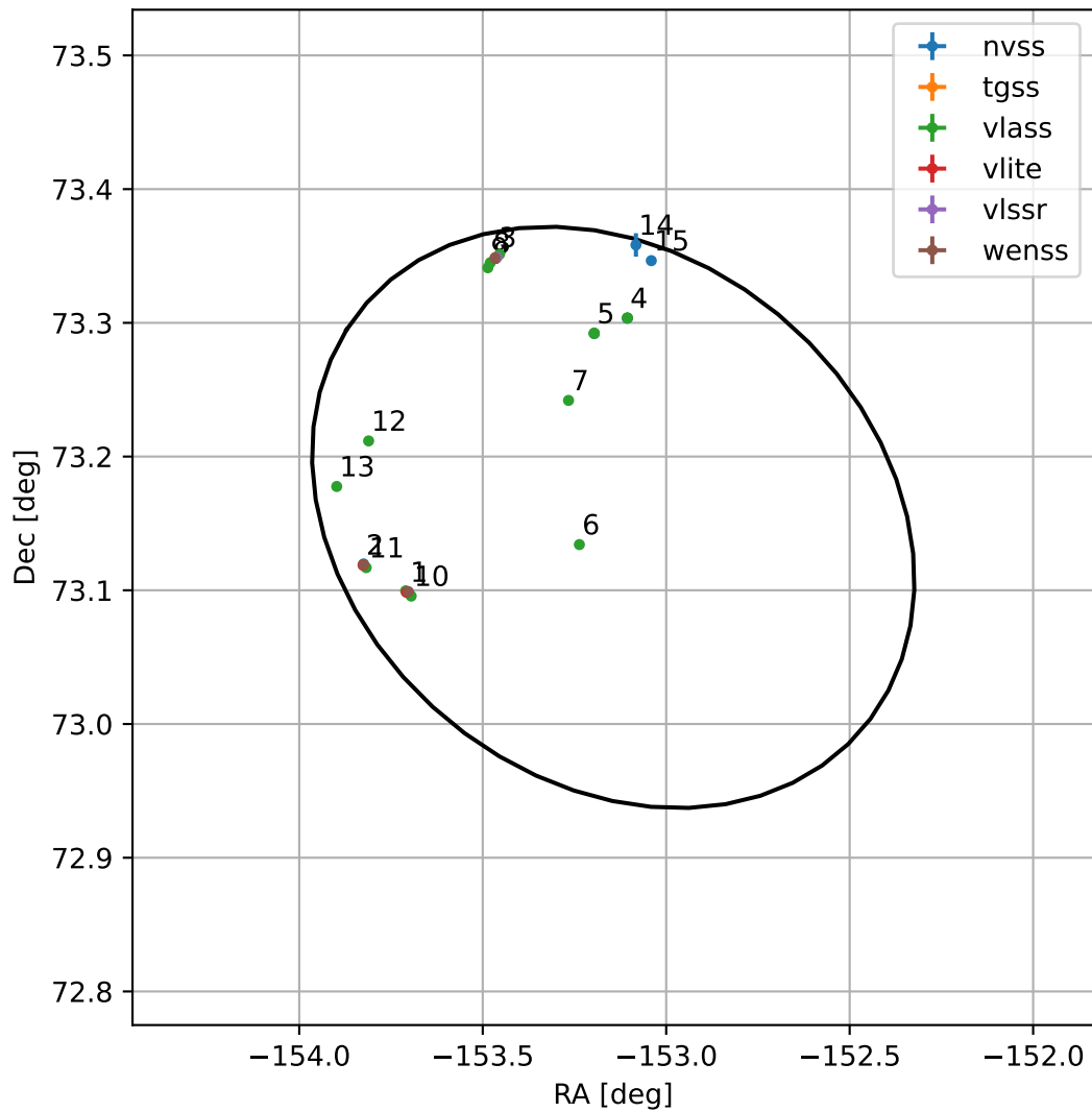
4FGL J1347.4+7309
