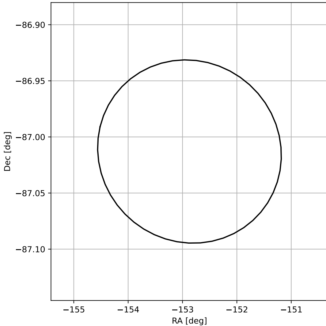
4FGL J1348.5-8700
