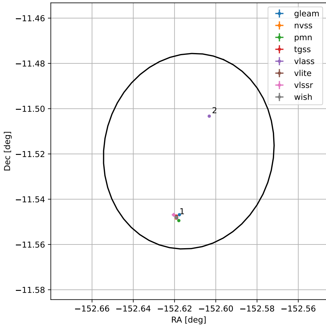
4FGL J1349.5-1131
