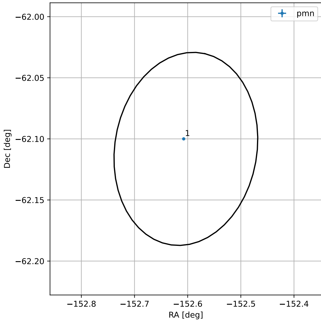
4FGL J1349.5-6206
