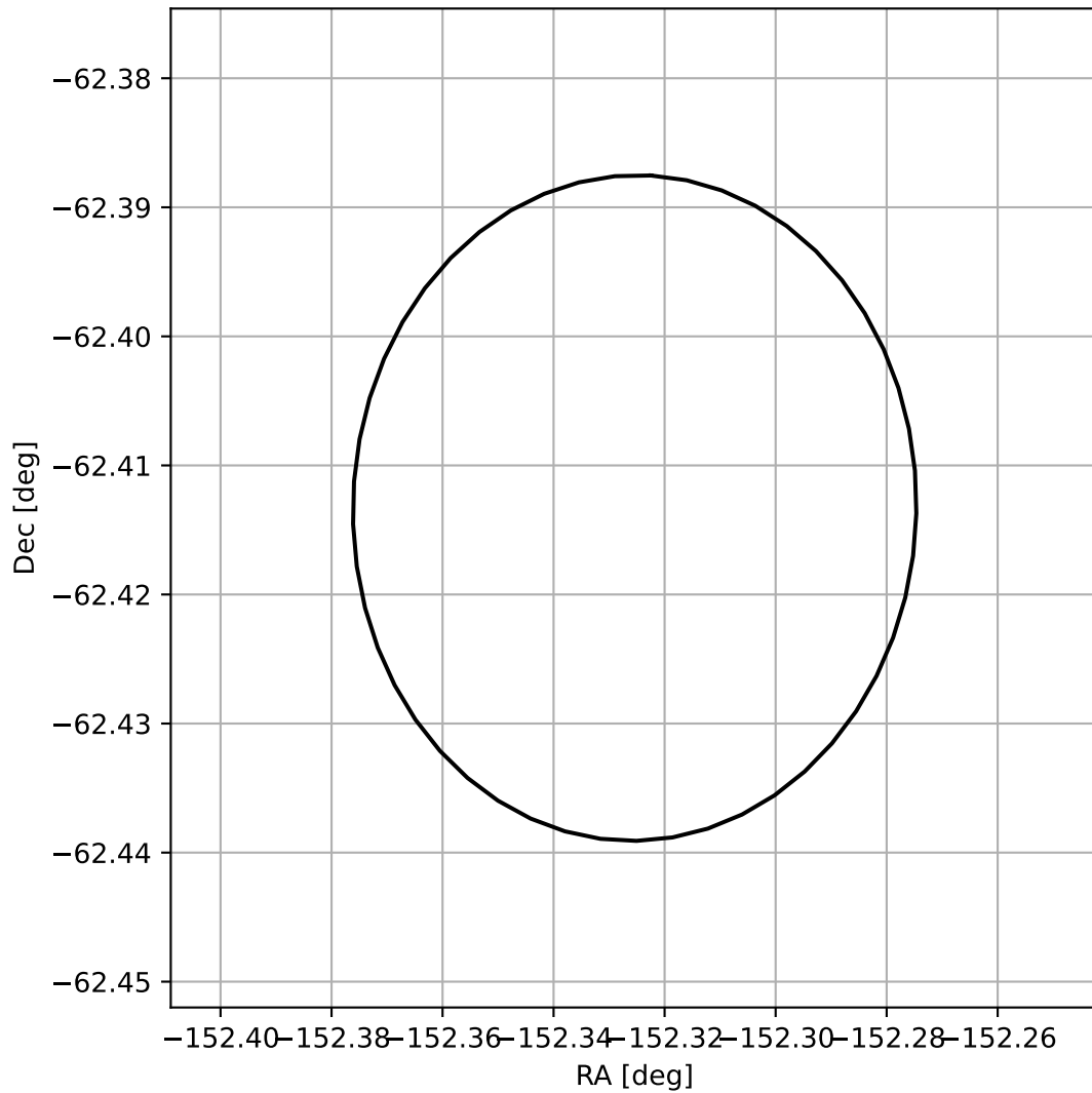
4FGL J1350.6-6224
