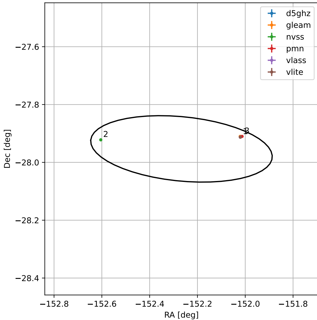
4FGL J1350.9-2757
