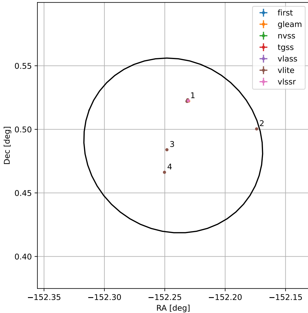
4FGL J1351.0+0029
