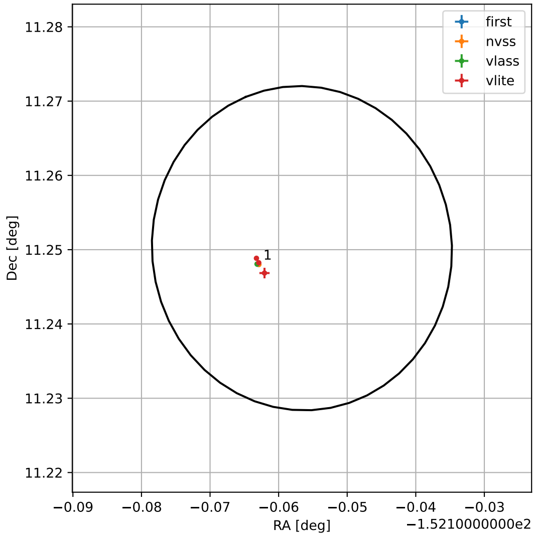
4FGL J1351.3+1115
