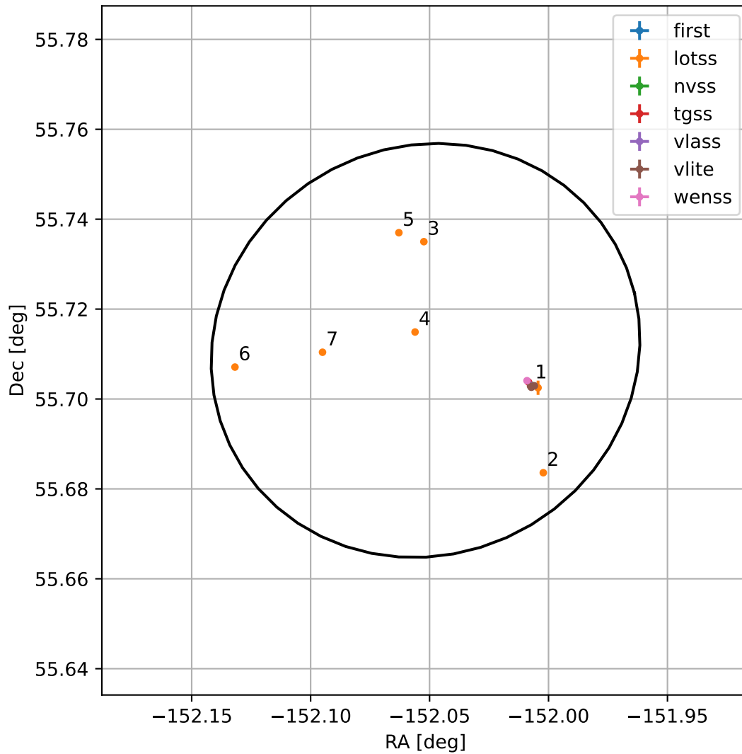
4FGL J1351.7+5542
