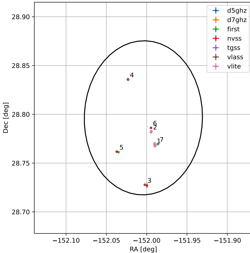
4FGL J1351.9+2847
